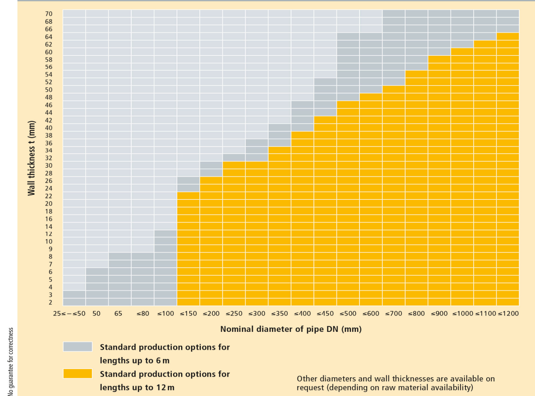
Fig. 1.1.1_1: Production possibilities for pipes from plate (without considering production with optional circumferential welds)
